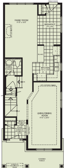
GROUND FLOOR ELEVATION A
