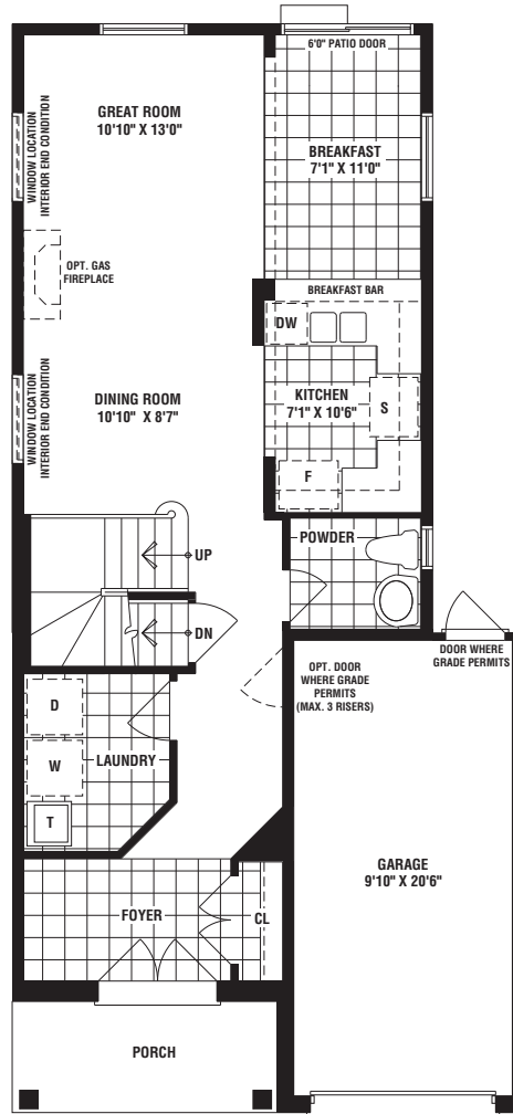
GROUND FLOOR ELEV. 'A' & 'B'
