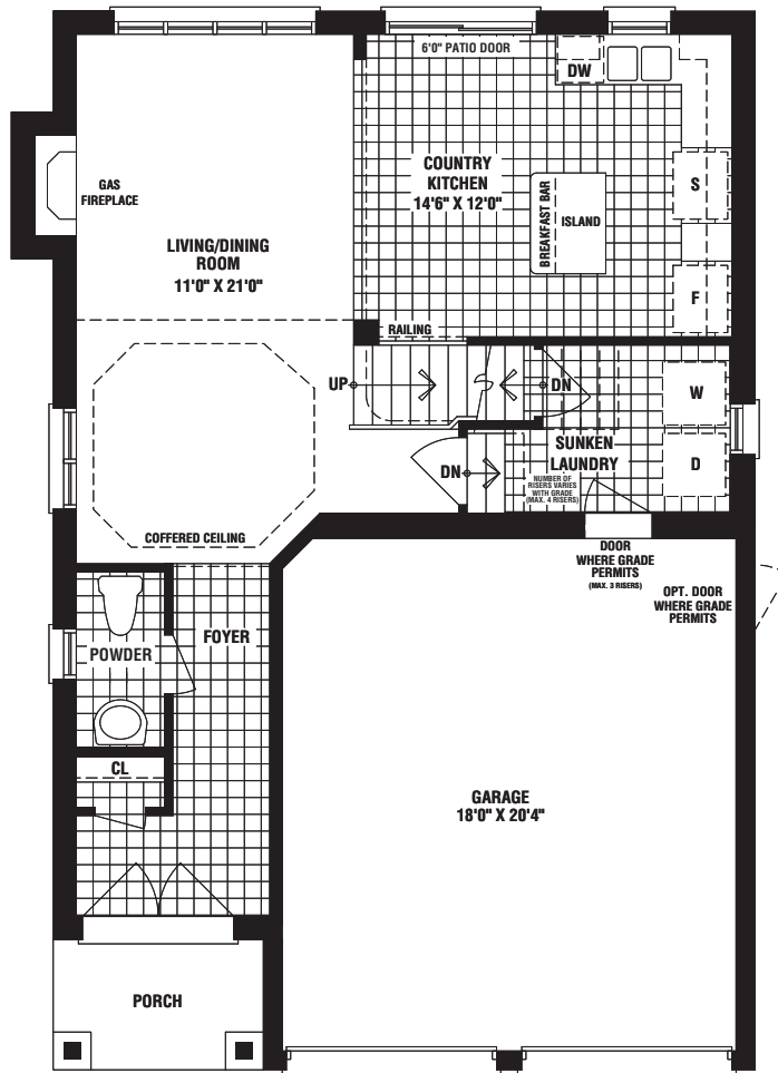
GROUND FLOOR 9'0" CEILING
