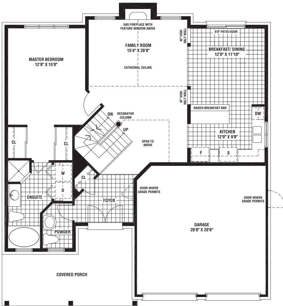
GROUND FLOOR ELEV. 'A'
