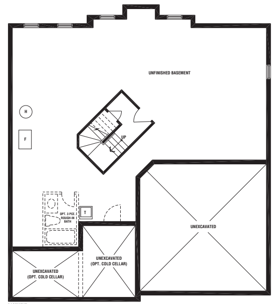
BASEMENT ELEV. 'K'
